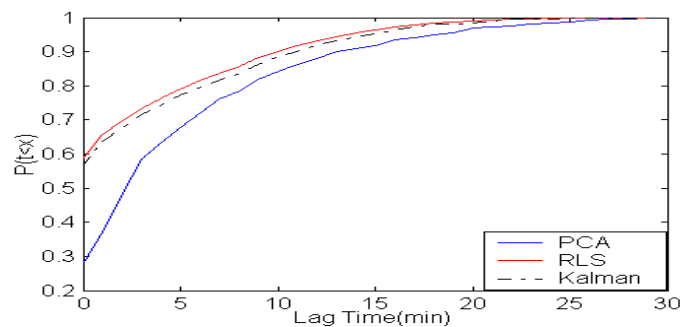
Fig. 16. Cumulative distribution function of detection lag time
