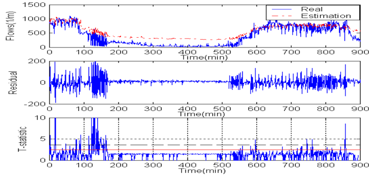
Fig. 8. Kalman-based method to detect original IF flow
