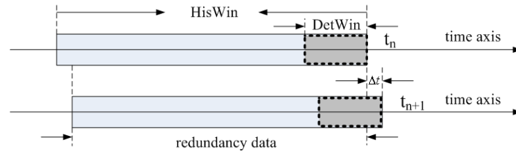
Fig. 5. Sliding window's variance ratio detection
